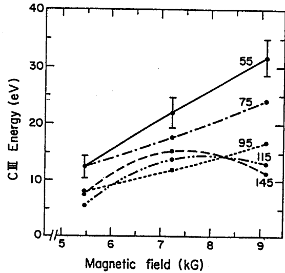
Fig. 3. Experimental data of the ion energy versus magnetic field intensity (taken from [3]).
