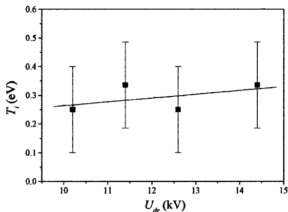
FIG. 7. Dependence of the plasma ion temperature on the driving pulse amplitude. \tau_{frame} = 5 \mu s .
